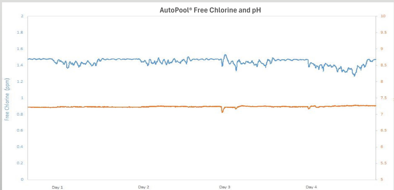
FIG. 2- pH AND CHLORINE DATA RECORDED BY THE AUTOPOOL® INSTALLED AT CROW WOOD LEISURE
