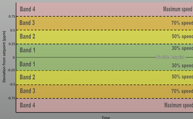
FIG. 1- HOW CHLORINE LEVELS CAN BE CONTROLLED BY VARYING PUMP SPEEDS
